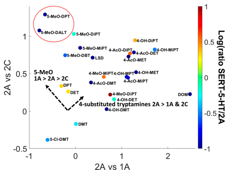
Fig. 7. Integrating patterns of selectivity of substituted tryptamines. A number of tryptamines that are selective for 5-HT 2A R receptors are also either nonselective for 5-HT 2A R vs. SERT or prefer SERT (see compounds marked with warmer colors to indicate those that do not prefer 5-HT 2A R vs. SERT). The N,N -substituted tryptamines that were tested (DMT, DET, and DPT) are all relatively nonselective for 5-HT 2A R vs. SERT. There are several compounds, typically 4-substituted, that exhibit selectivity for 5-HT 2A R vs. 5-HT 1A R and 5-HT 2C R and vs. SERT. The 5-MeO compounds tested prefer 5-HT 2A R relative to SERT.
