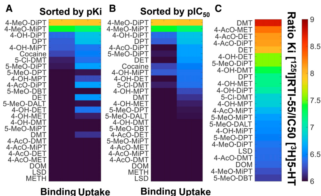
Fig. 5. Substituted tryptamines sorted by pK_i and pIC_{50} at SERT to show relative affinity and potency. (A) Substituted tryptamines were sorted by pK_i of [^{125}I]RTI-55 binding or (B) sorted by pIC_{50} of [^3H]5-HT uptake at SERT. pK_i or pIC_{50} of the partner assay ( [^3H]5-HT uptake for (A) and [^{125}I]RTI-55 binding for (B)) were included alongside the sorted column. Of the tryptamines tested, 4-MeO-substituted tryptamines exhibit the highest binding at the RTI-55 and 5-HT uptake sites on SERT. Other 4-substituted N,N -diisopropyl and non-ring-substituted N,N -diethyl tryptamines predominantly exhibit binding to the [^3H]5-HT site of SERT. (C) Substituted tryptamines were sorted by the ratio of K_i vs. [^{125}I]RTI-55 and IC_{50} vs. [^3H]5-HT at SERT. Of the tryptamines tested, 4-AcO-substituted compounds and those with only N,N -substitutes exhibited the highest ratios of K_i at the [^{125}I]RTI-55 binding site on SERT vs. IC_{50} competing against [^3H]5-HT . Compounds with higher ratios are more substrate-like at SERT.
