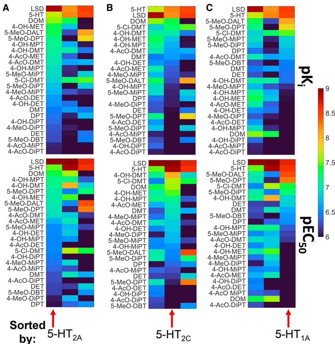
Fig. 4. Substituted tryptamines sorted by pK_i and pEC_{50} for 5\text{-HT}_{2A}R (A), 5\text{-HT}_{2C}R (B), and 5\text{-HT}_{1A}R (C) to show ordered relative affinities (top row) and relative potencies (bottom row) for all compounds to emphasize any chemical bases for affinity and potency. (A) Both 4- and 5-substituted tryptamines exhibit a broad range of affinities and potencies for 5\text{-HT}_{2A}Rs depending on the N,N substitutions (left panel). (B) 5-MeO and N,N DiPT-substituted tryptamines exhibit the lowest affinities and potencies for 5\text{-HT}_{2C}Rs (middle panel). (C) 5-MeO- and N,N -substituted tryptamines exhibit highest affinities and potencies for 5\text{-HT}_{1A}Rs (right panel).
